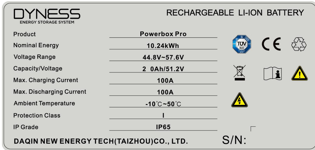
Figure 1-1 Battery Energy Storage System nameplate
